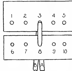
FIG. 224. STRAIGHT STITCH BELT LACING, GRAIN SIDE.
